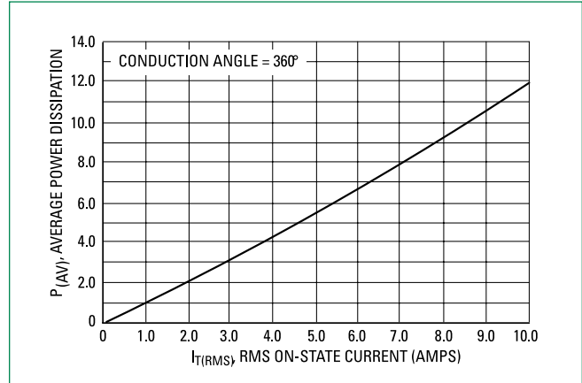
Figure 2. Power Dissipation
