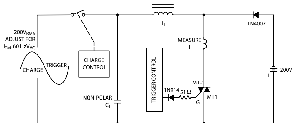
Figure 10. Simplified Test Circuit to Measure the Critical Rate of Rise of Commutating Current ( di/dt )
