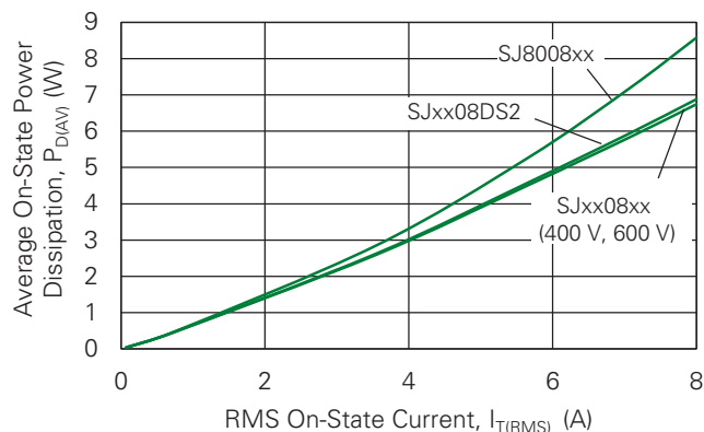
Fig. 6. Typical Power Dissipation vs. RMS On-state Current
