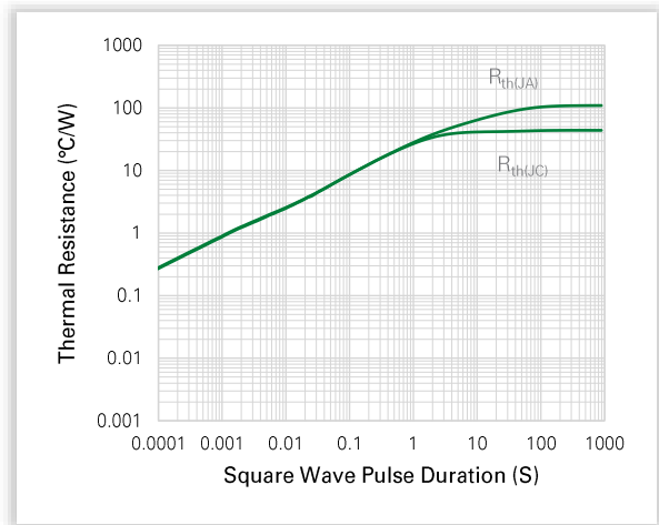
Figure 9. Thermal Resistance (°C/W) vs. Square Wave Pulse Duration (S)
