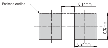
Recommended soldering pad layout
