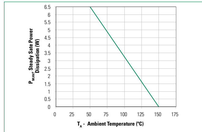
Figure 6 - Steady State Power Dissipation Derating Curve
