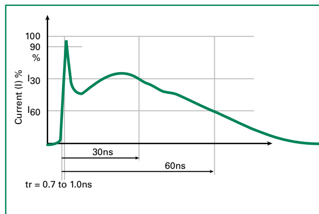
Figure 1. ESD Test Waveform
