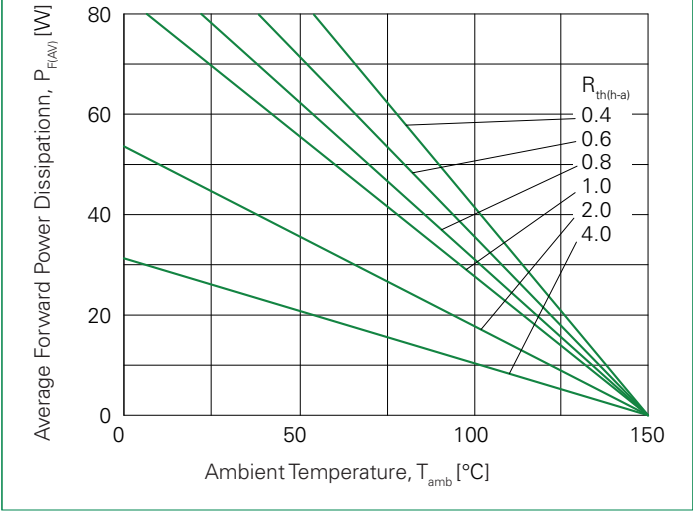
Fig. 8. Average Forward Power Dissipation vs. Ambient Temperature
