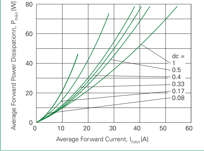
Fig. 7. Average Forward Power Dissipation vs. Mean Forward Current
