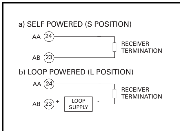
FIGURE 3.2 Analog-Output Connections.
