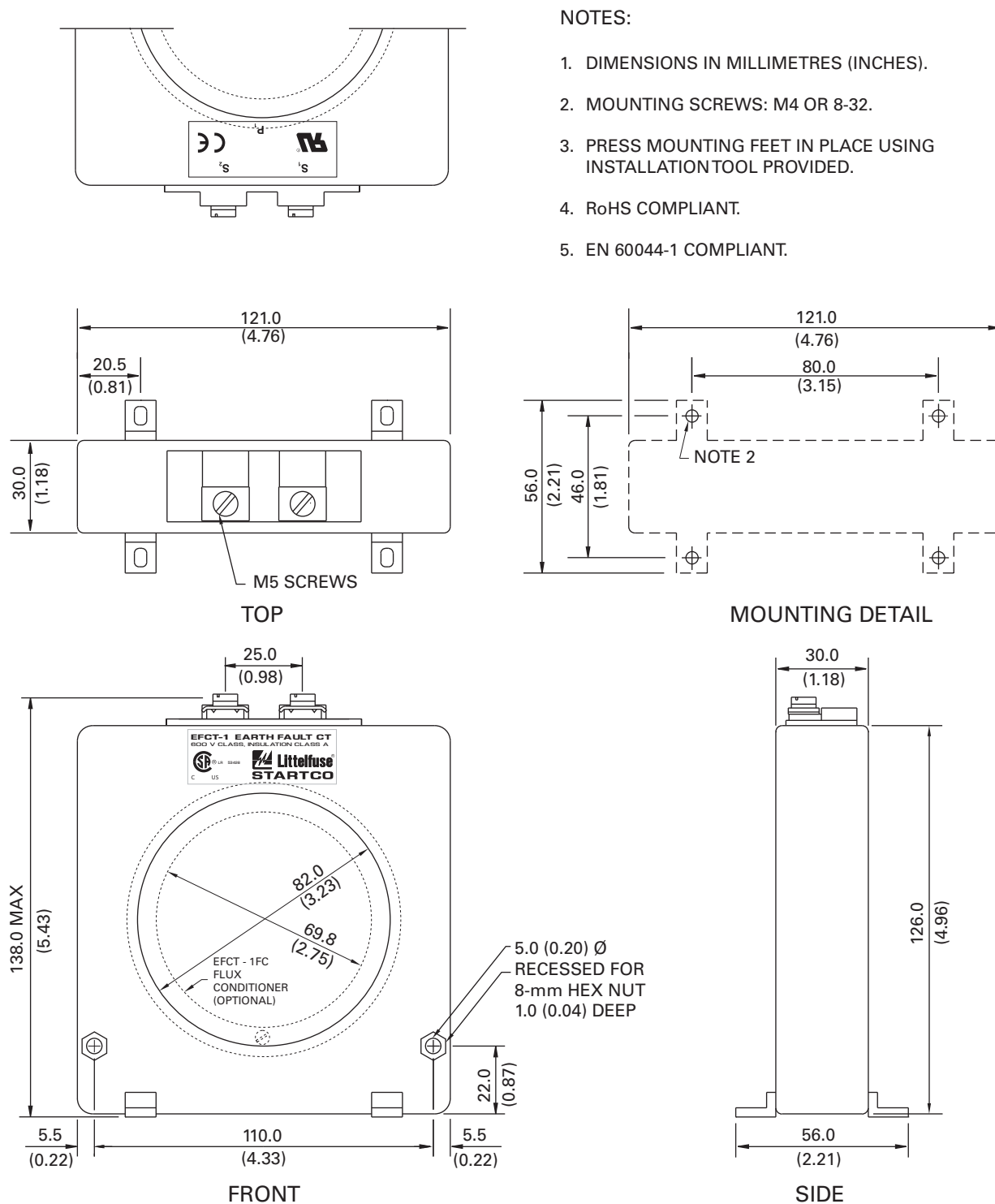
FIGURE 2.4 EFCT-1 Outline and Mounting Details.
