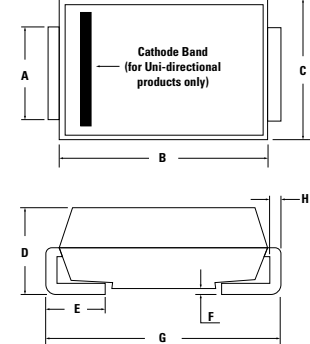
L003b DO-214A Weight = 0.2 g
