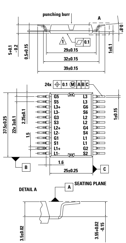
X026d ISOPLUS™-DIL (SMD) Weight = 13 g
