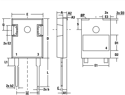
X016d ISO247™ Weight = 4 g
