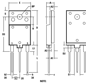
X017c TO-3PFP Weight = 5.5 g
