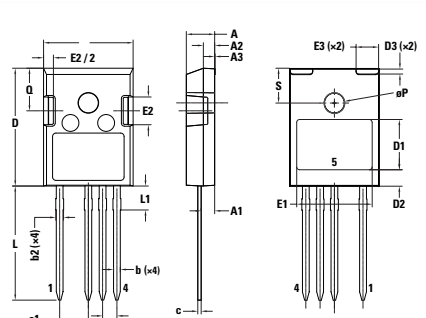
X016f ISO247™ Weight = # g
