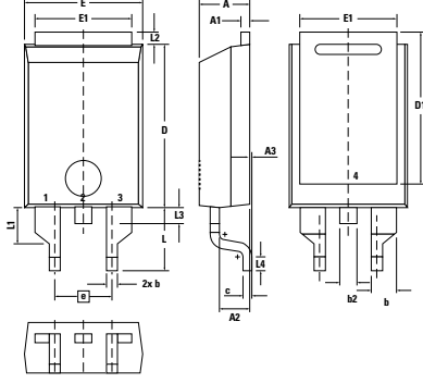
X013 PLUS220™ (SMD) Weight = 2 g
