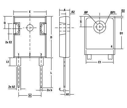
X014b TO-247 AD Weight = 6 g
