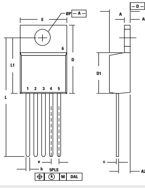
X006 TO-220 (5) Weight = 2 g
