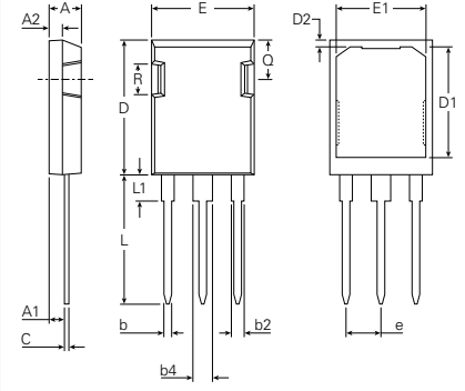
X015a PLUS247™ Weight = 7 g
