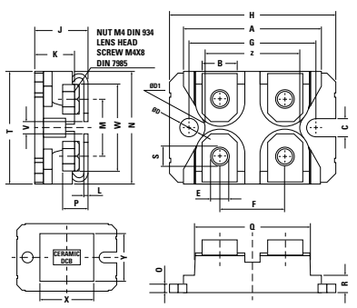
X028 ISOPLUS227™ Weight = 19 g
