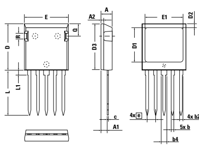
X024a ISOPLUS i4-PAC™ Weight = 6 g
