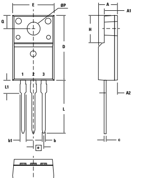
X007a TO-220 ABFP Weight = 2 g
