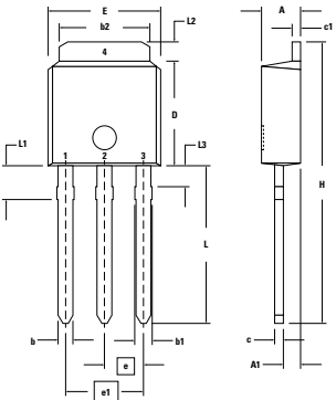
X003 TO-251 AA Weight = 0.4 g
