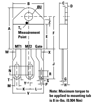
L002a TO-218 x Weight = 5.2 g
