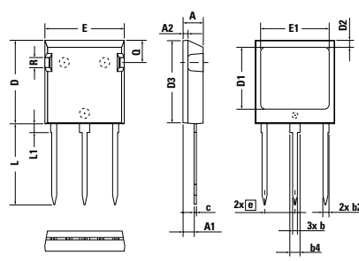
X024b ISOPLUS i4-PAC™ Weight = 5.5 g
