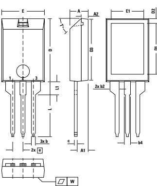
X010a ISOPLUS220™ AB Weight = 2.5 g
