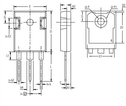
X014a TO-247 AD Weight = 6 g
