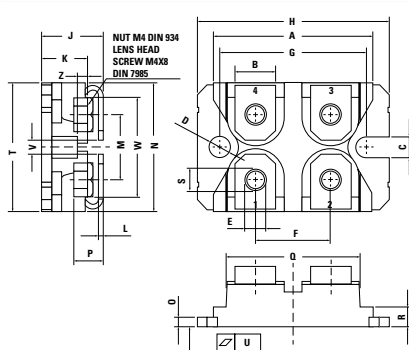
X027a SOT-227 B miniBLOC Weight = 29 g
