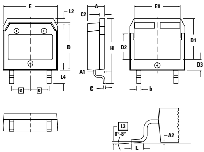
X019a TO-268 AA (D3PAK HV) Weight = 4 g
