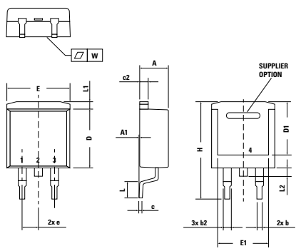
X011b TO-263 AB (D2PAK) Weight = 1.5 g
