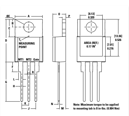
L005c TO-220AB (ISO) Weight = 2 g
