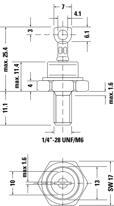
X206a DO-203 AB [UNF] (DO-5) X206b DO-203 AB [M] (DO-5) Weight = 14 g
