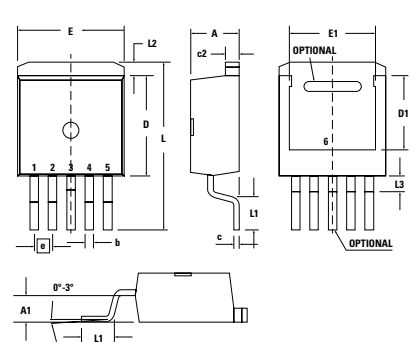
X012a TO-263 (5) Weight = 1.5 g
