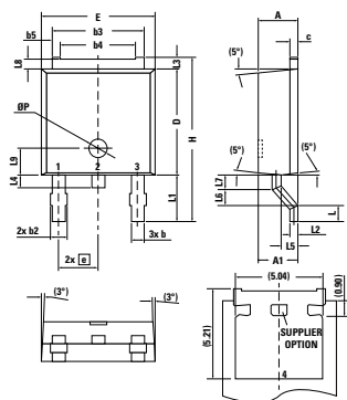
X004 TO-252 AA (D PAK) Weight = 0.3 g
