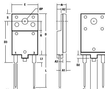
X017d TO-3PFP Weight = 5.4 g
