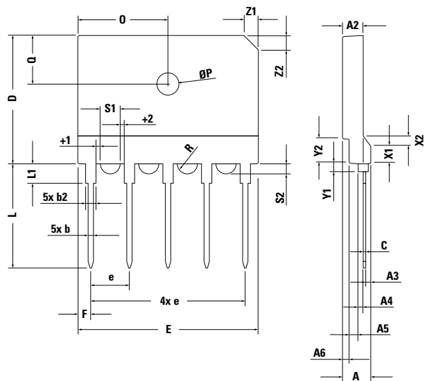
X025b GUPF Weight = 8.5 g
