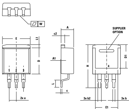
X011a TO-263 AA (D2PAK) Weight = 1.5 g
