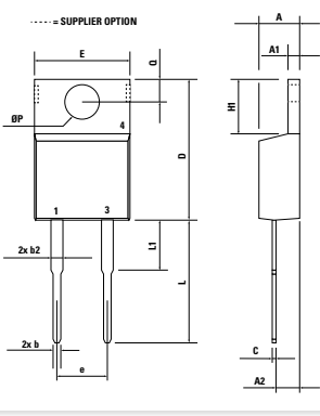
X005b TO-220 AB Weight = 2 g
