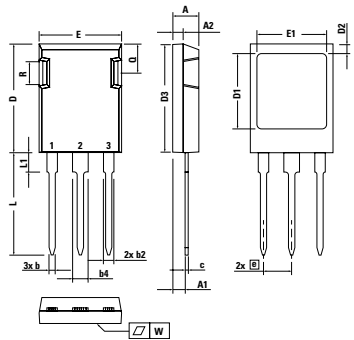
X016a ISOPLUS247™ Weight = 4.5 g
