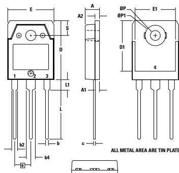
X017a TO-3P Weight = 5.5 g
