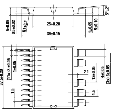
X026c ISOPLUS™-DIL (SMD) Weight = 13 g
