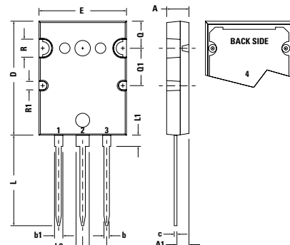
X021a PLUS264™ Weight = 10 g
