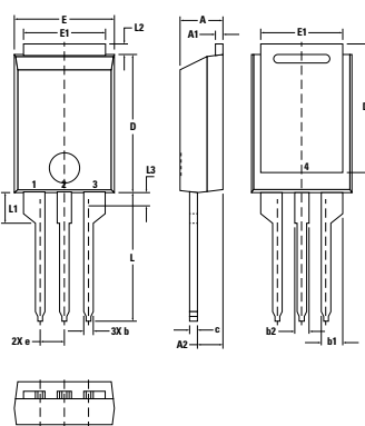
X009a PLUS220™ Weight = 2.5 g b) middle leg cut
