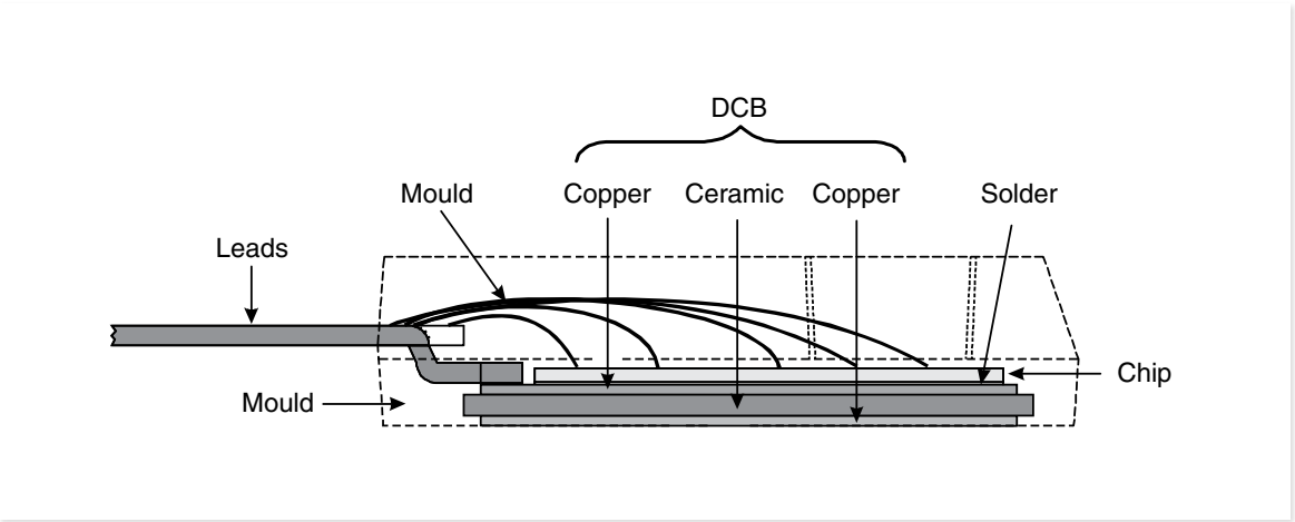
Package Cross-Section
