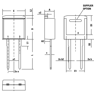
X008b TO-262 I2PAK Weight = 1.5 g
