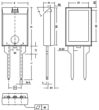
X010b ISOPLUS220™ AC Weight = 2.5 g
