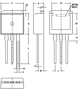
X008a TO-262 I2PAK Weight = 1.5 g
