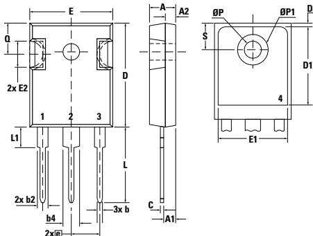
L014a TO-247AD Weight = 6 g
