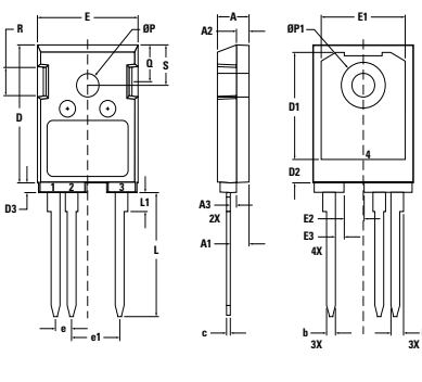
X014c TO-247 AD Weight = 6 g
