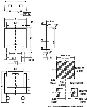
X004a TO-252 AA (D PAK HV) Weight = 0.3 g
