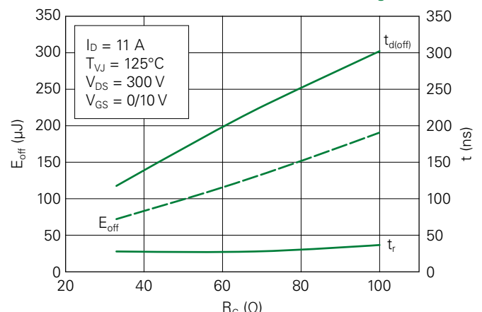
Fig. 12. Typical Turn-off Energy and Switching Times vs. Gate Resistance, Inductive Switching
