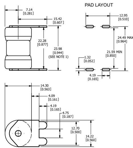
Solder Mount - LSE Version
