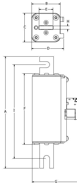
Figure 3. DIN-blade style
