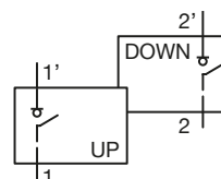
Type CB (2 Pole)
