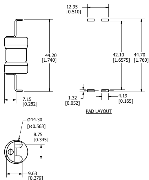
Solder Mount - MB Version
