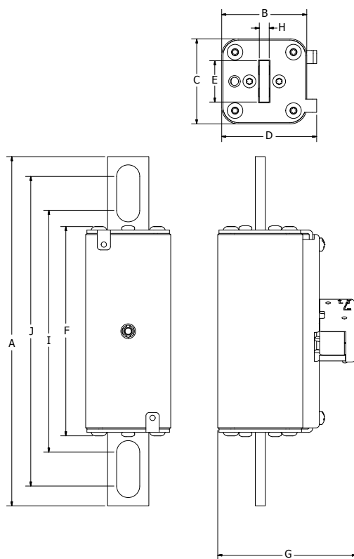
Figure 2. Bolted-blade style
