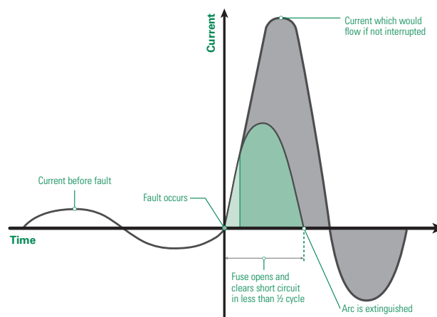
Figure 13 – Current-limiting Fuse
