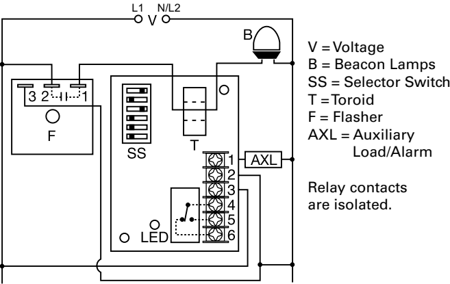
BEACON LAMP CONNECTION DIAGRAM
