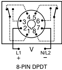
8-PIN DPDT
