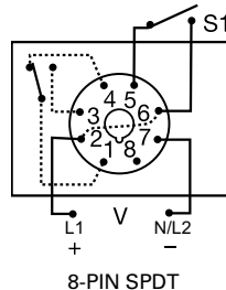
8-PIN SPDT
