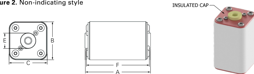
Figure 2. Non-indicating style
