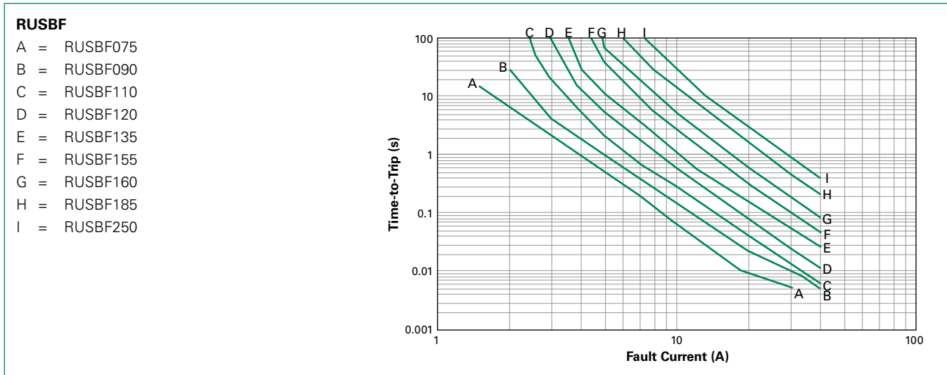
Typical Time-to-Trip Curves at 20°C
