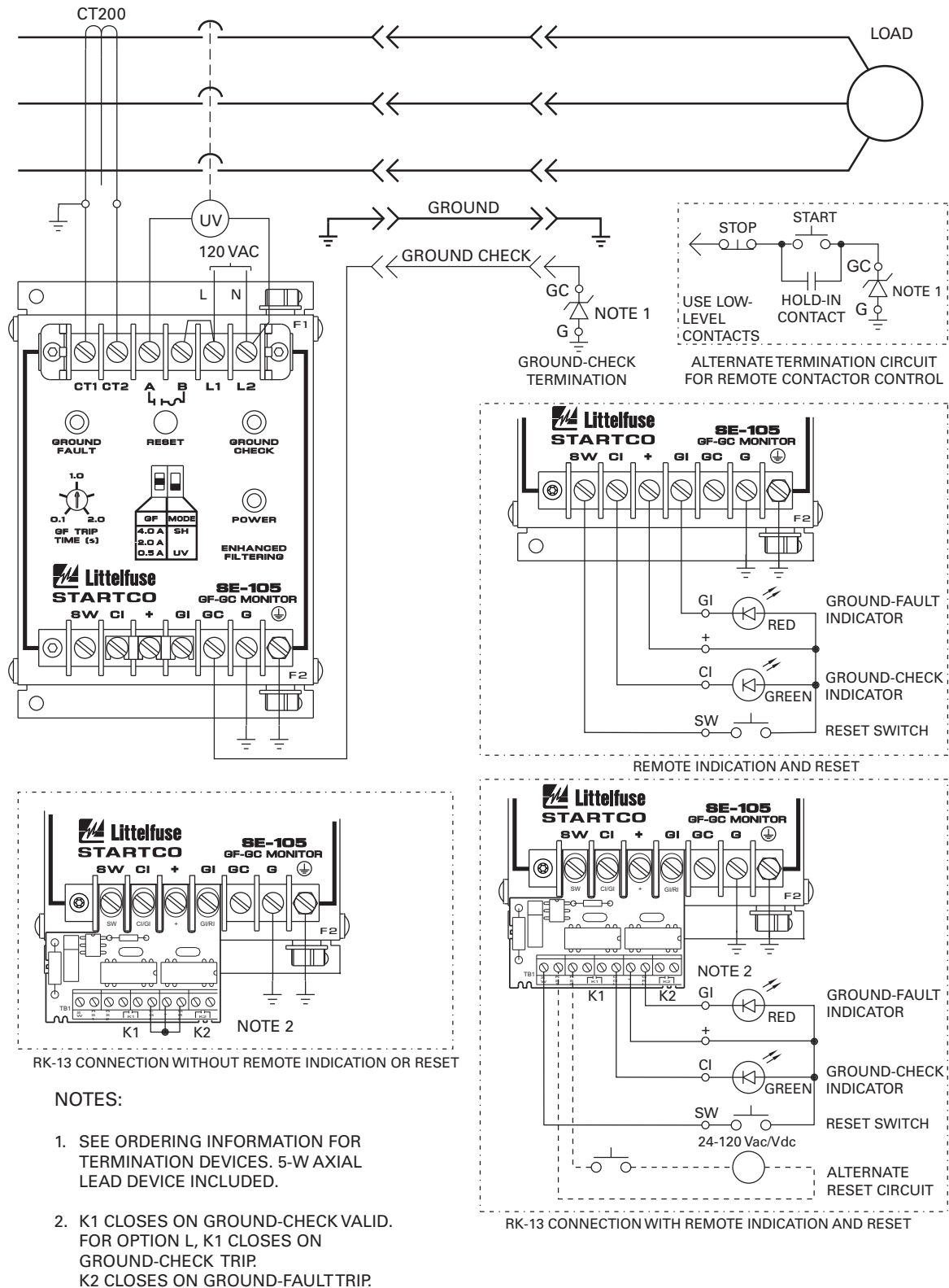
FIGURE 1. Typical Application.
