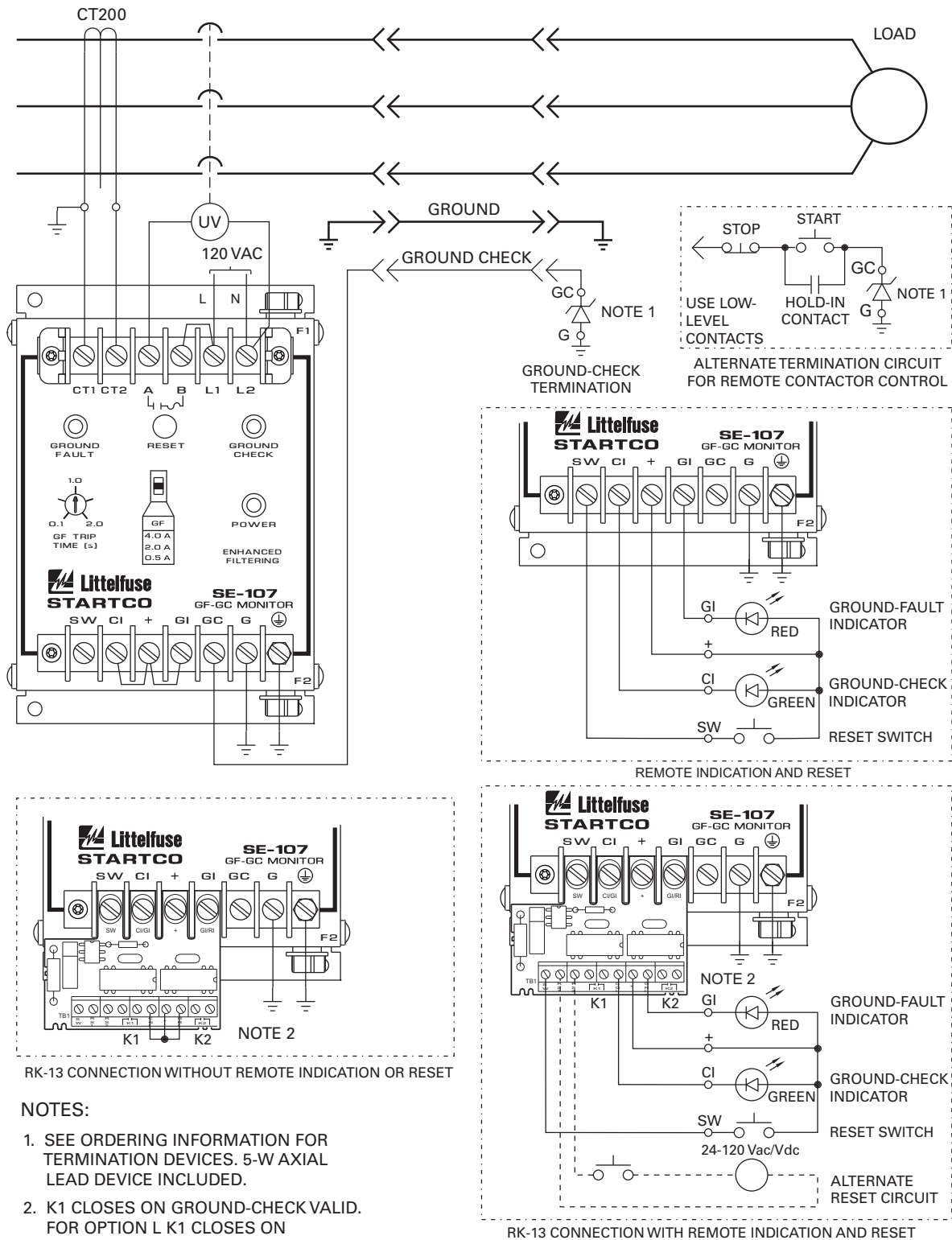
FIGURE 1. Typical Application.
