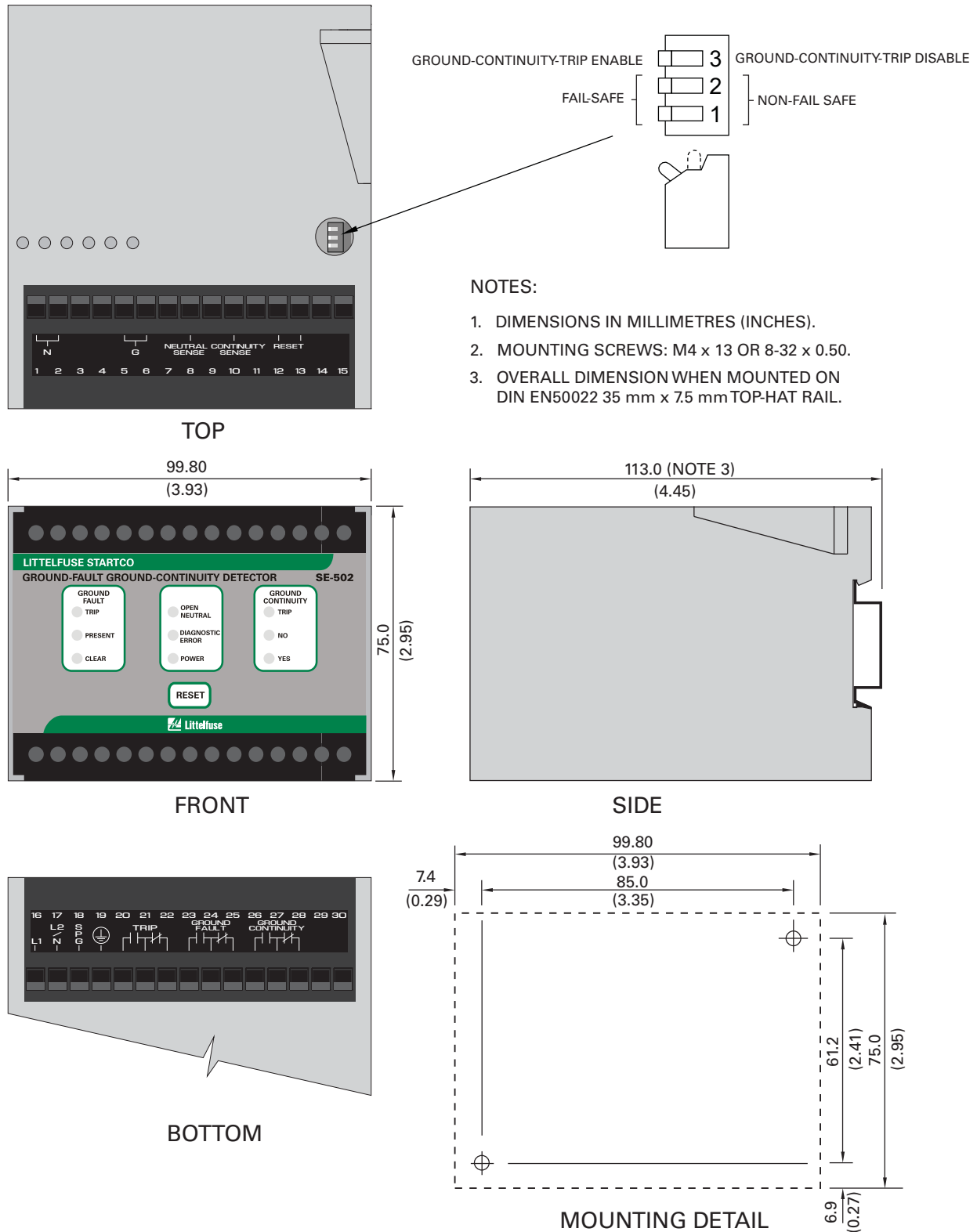
FIGURE 1. SE-502 Outline and Mounting Details.
