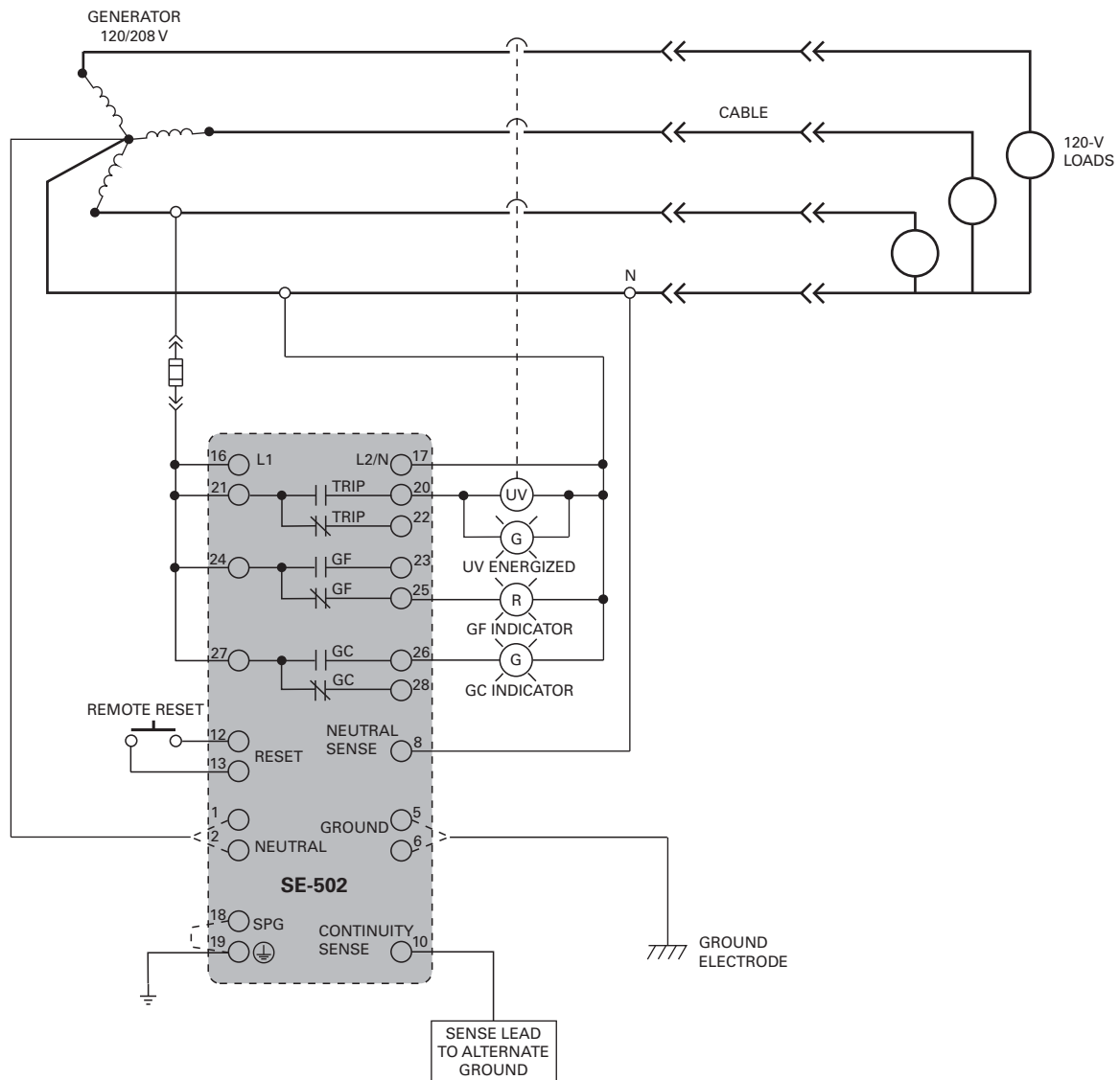
FIGURE 2. SE-502 Typical Application.
