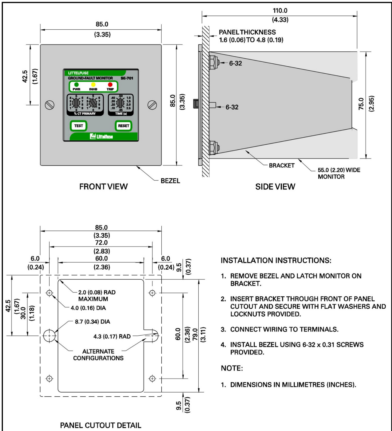
FIGURE 8 PMA-55 Panel-Mount Adapter.
