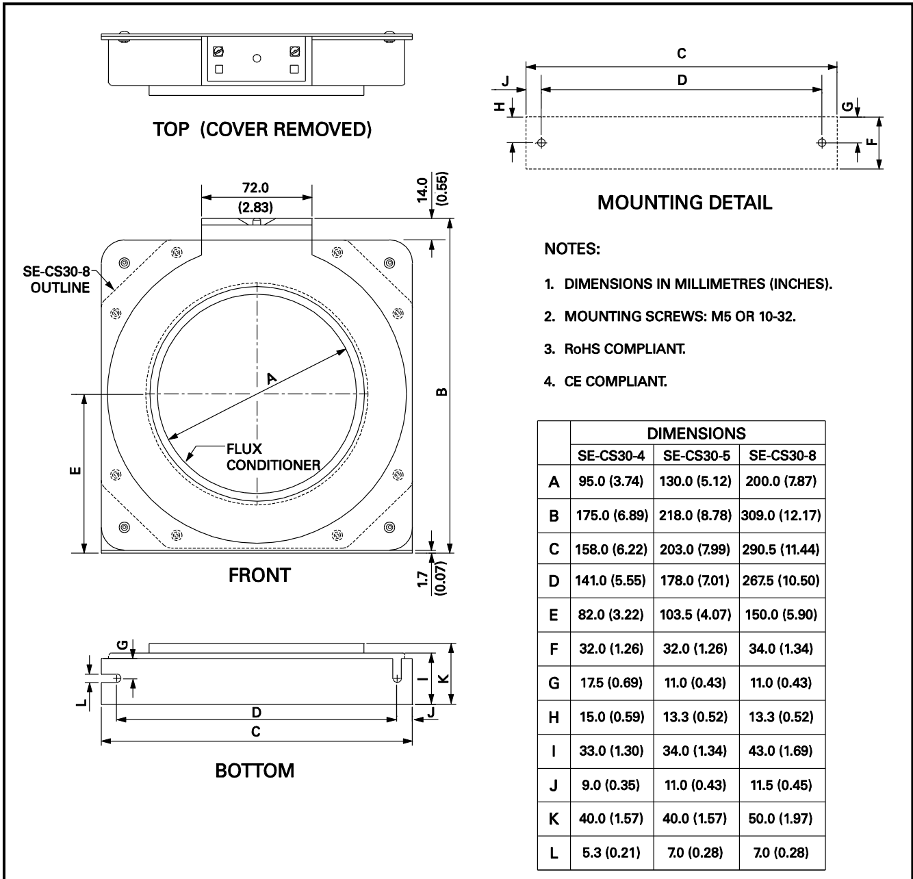
FIGURE 7. SE-CS30-4, -5, and -8 Current Sensors
