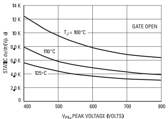
Figure 9. Exponential Static dv/dt vs. Peak Voltage, MT2(-)
