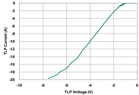
Negative Transmission Line Pulsing (TLP) Plot
