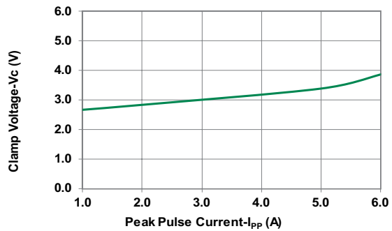
Clamping Voltage vs. Peak Pulse Current
