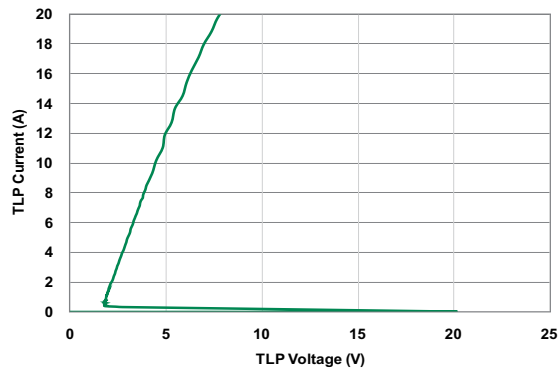
Positive Transmission Line Pulsing (TLP) Plot
