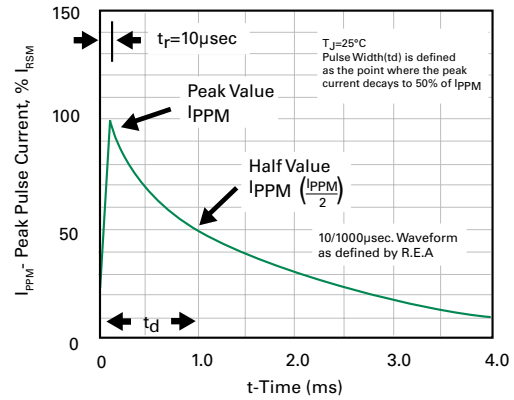
Figure 4 - Pulse Waveform
