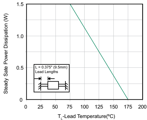
Figure 6 - Steady Pulse Derating Curve
