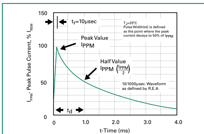
Figure 3 - Pulse Waveform
