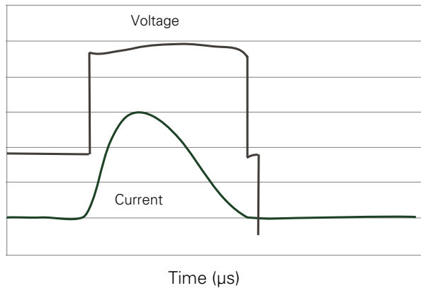
Figure 3 - Surge Response (8/20 Surge current waveform)
