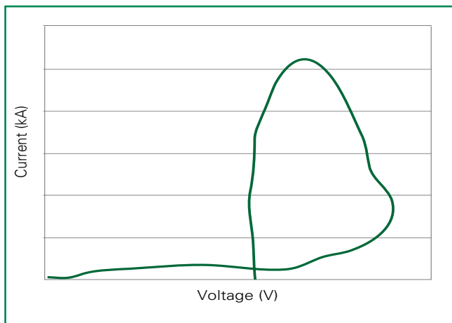
Figure 2 - Surge Response
