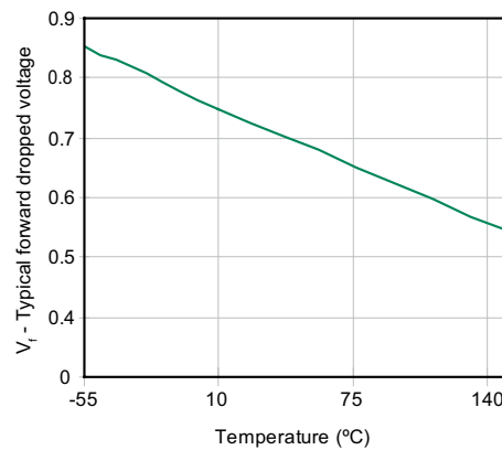
Figure 6 - Forward Voltage
