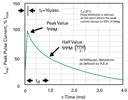
Figure 4 - Pulse Waveform - 10/1000 \mu\text{s}
