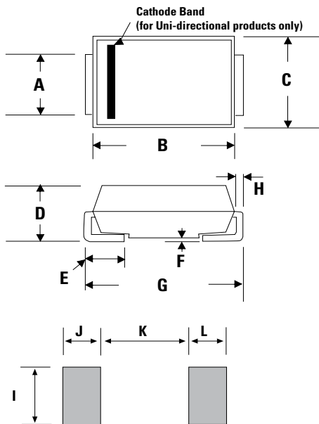
Solder Pads (all dimensions in mm)
