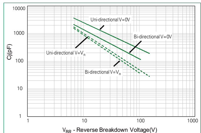
Figure 8 - Typical Junction Capacitance
