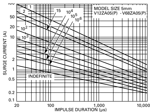
Figure 14 SURGE CURRENT RATING CURVES FOR
