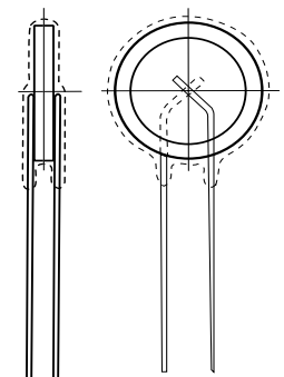
FIGURE 9B. CROSS-SECTION OF RADIAL LEAD PACKAGE
