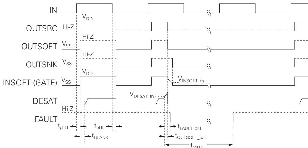
Figure 2 Logic Diagram
