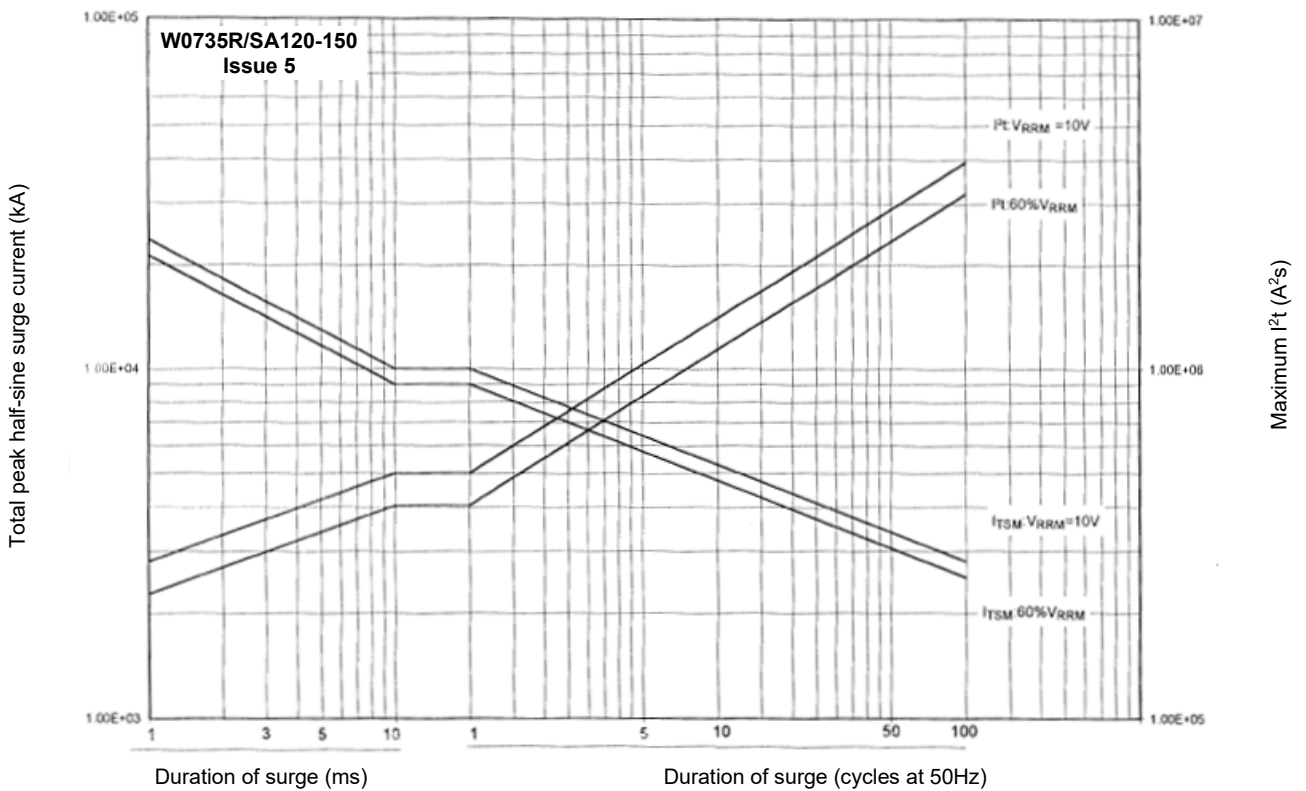
Figure 5 – Maximum non-repetitive surge current at initial junction temperature 190°C
