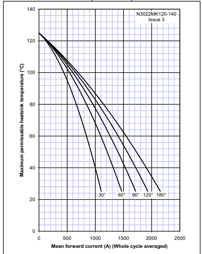
Figure 13 – On-state current vs. Heatsink temperature – Cathode Side Cooled (Sine wave)
