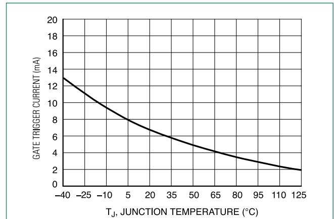
Figure 4. Typical Gate Trigger Current vs Junction Temp
