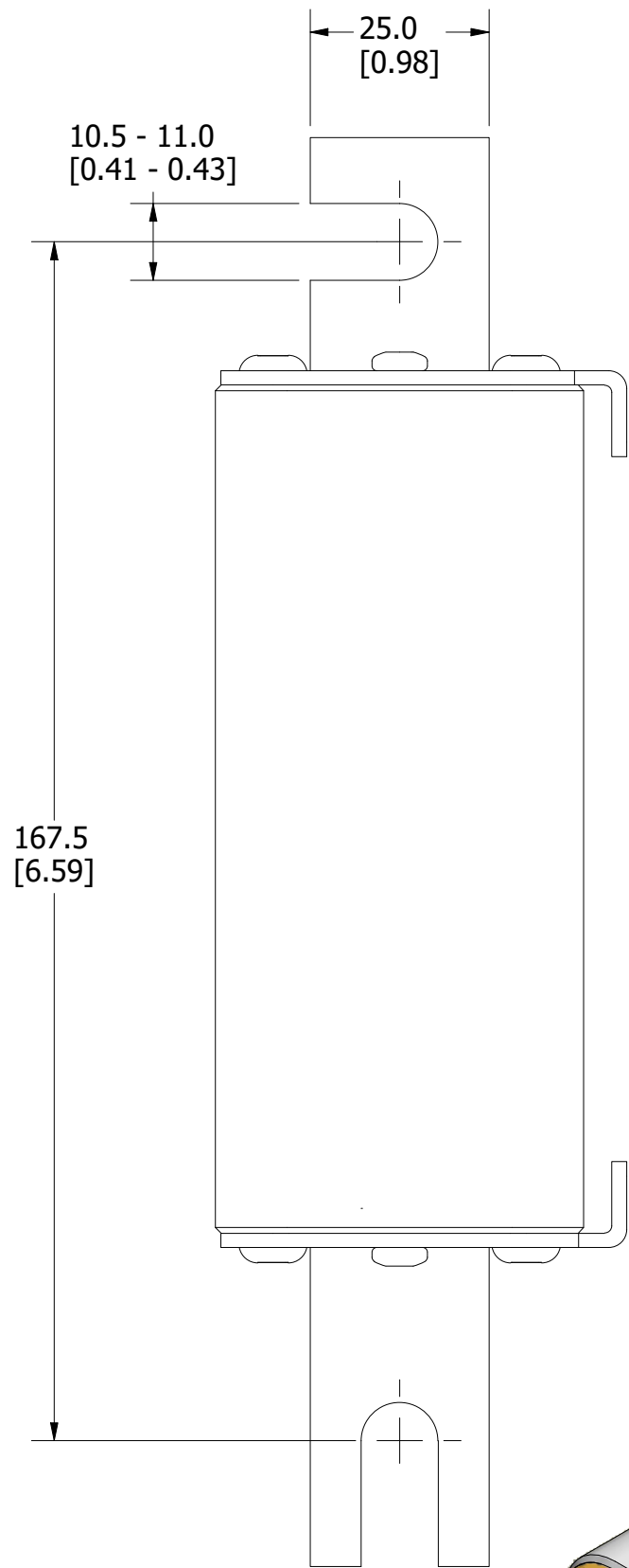
FUSE
