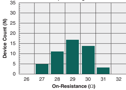
Typical On-Resistance Distribution (N=50, I_F=2mA , I_L=100mA )
