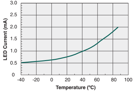
Typical I_F for Switch Dropout vs. Temperature ( I_L=50mA )
