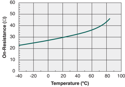
Typical On-Resistance vs. Temperature ( I_F=10mA, I_L=50mA )
