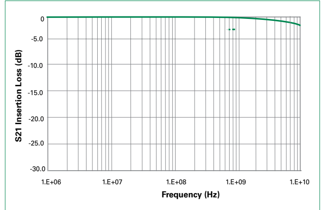
Insertion Loss Diagram - Bidirectional
