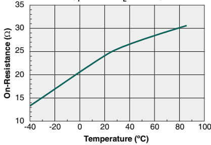
Typical On-Resistance vs. Temperature ( I_F=10mA, I_L=80mA )
