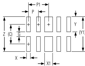
Alternative Soldering Pad Layout
