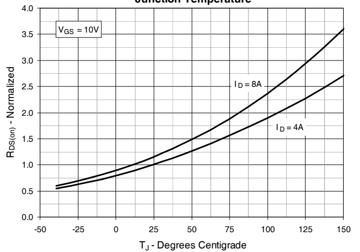
Fig. 4. R_{DS(on)} Normalized to I_D = 4A Value vs. Junction Temperature
