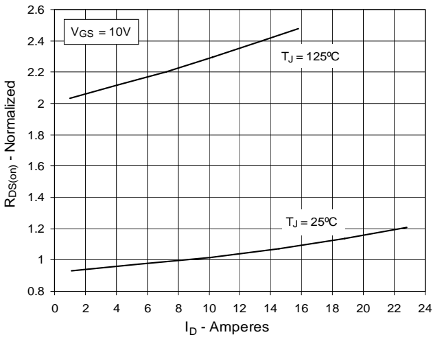
Fig. 5. R_{DS(on)} Normalized to I_D = 8\text{A} Value vs. Drain Current
