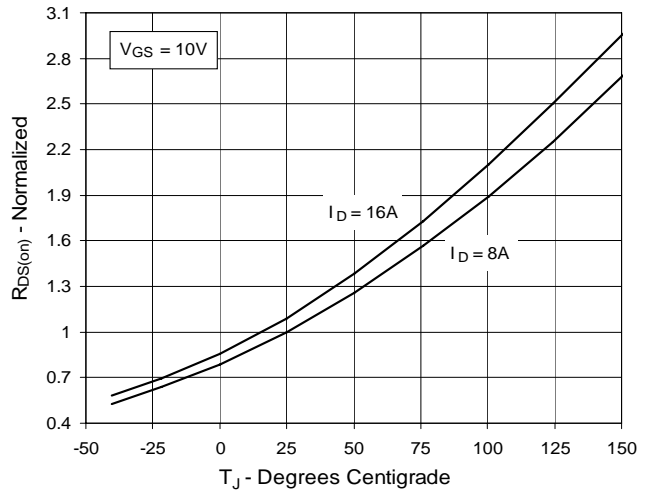
Fig. 4. R_{DS(on)} Normalized to I_D = 8\text{A} Value vs. Junction Temperature
