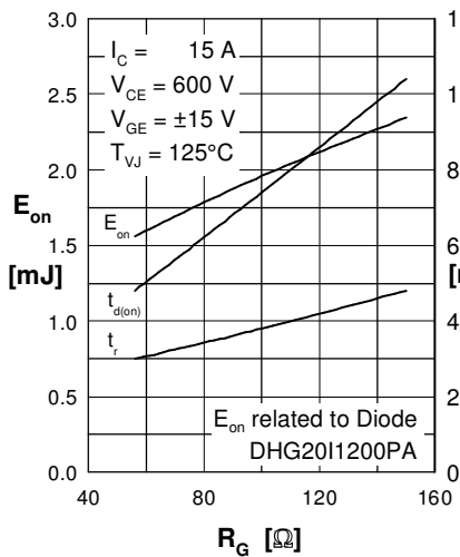
Fig. 7 Typ. switching energy vs. gate resistance
