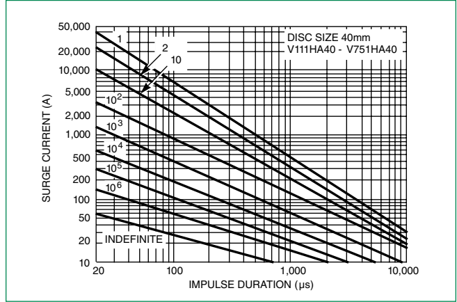
Repetitive Surge Capability for 40mm Parts V111HA40 – V751HA40
