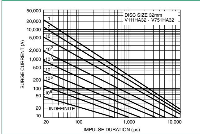
Repetitive Surge Capability for 32mm Parts V111HA32 – V751HA32
