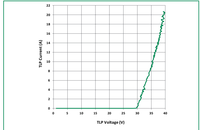
AQ24 Transmission Line Pulsing(TLP) Plot
