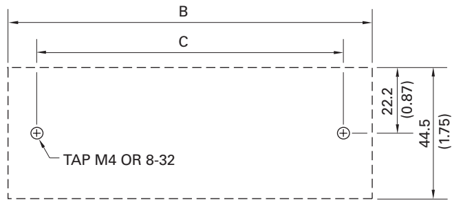
MOUNTING DETAIL
