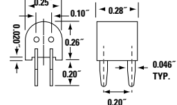
Circuit Board Mounting Detail
