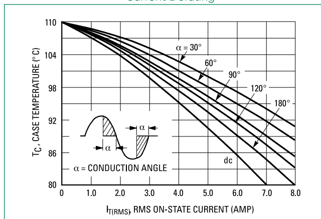
Figure 1. Current Derating
