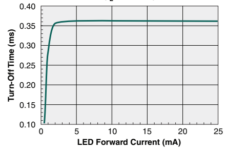
Typical Turn-Off Time vs. LED Forward Current ( I_L=120mA )
