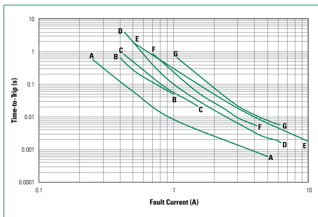
Typical Time-to-Trip Curves at 25°C
