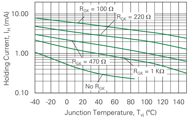
Fig. 12. Typical DC Holding Current with R_{GK} vs. Junction Temperature (Sensitive SCR)
