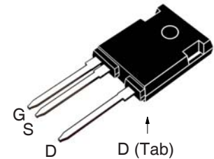
TO-247HV (IXTH)
