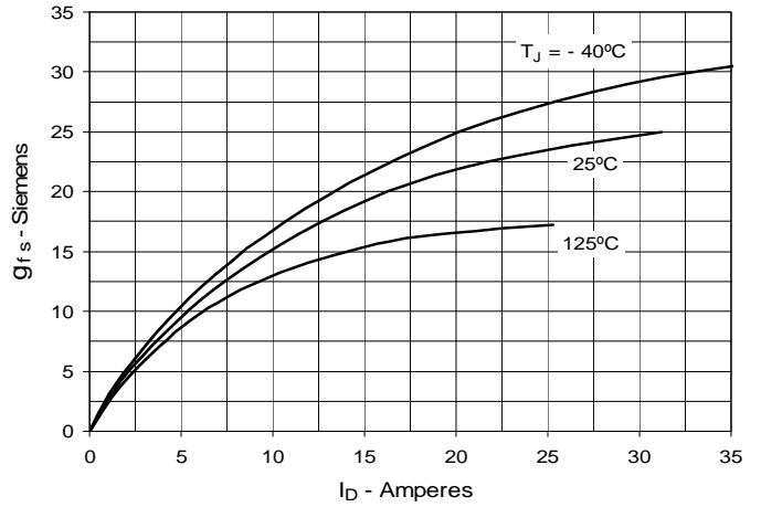
Fig. 8. Transconductance
